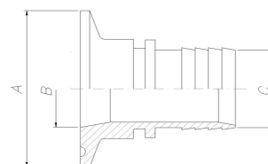
CLAMP 90°
